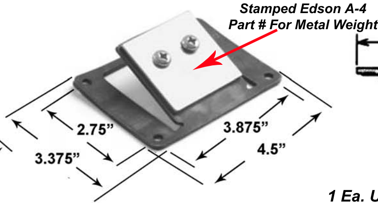
160-G-107 Side Inlet & Side Discharge Flapper Valve Assembly
