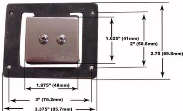
160-A-1207 Side Inlet & Side Discharge Flapper Valve Assembly
