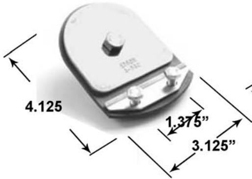
160-G-108 Bottom Inlet Flapper Valve Assembly
