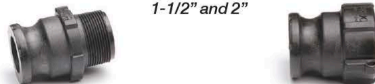
MALE NPT x MALE QC ADAPTER Order #157MM
